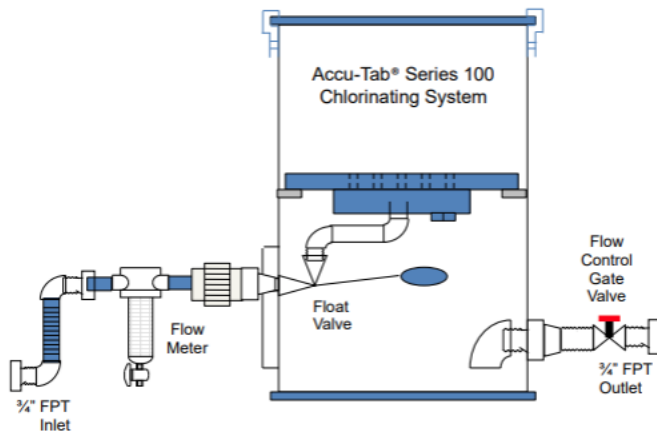
System Schematic - Accu-Tab® Series 100 Chlorination System when using Suction and Forced Venturi Return
