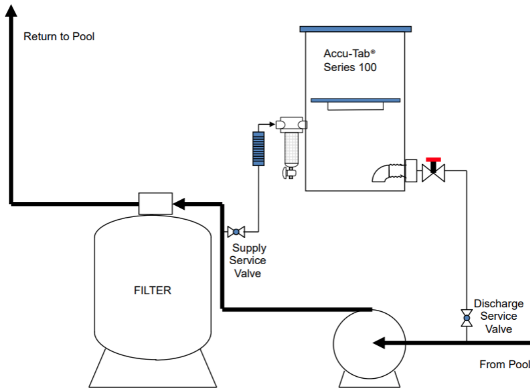
FIGURE 2 – Accu-Tab® Series 100 Chlorination System Suction Return Installation Example
