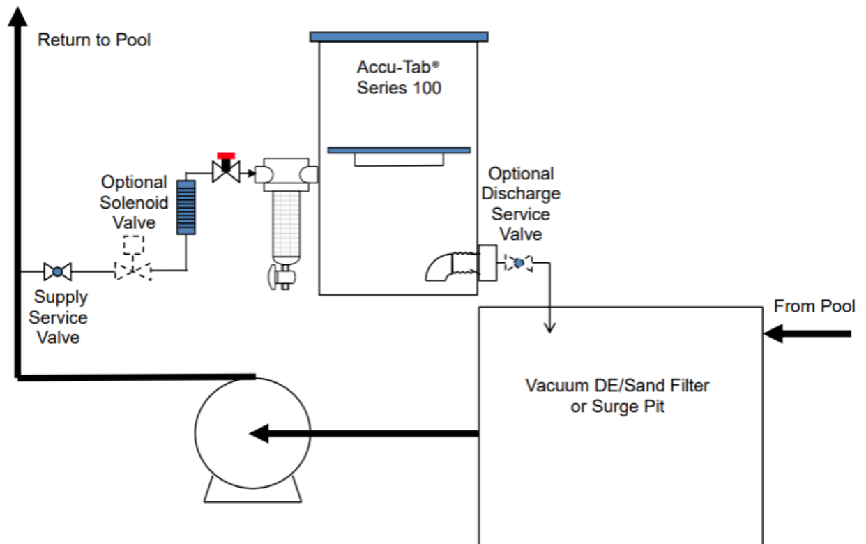
FIGURE 1 – Accu-Tab® Series 100 Chlorination System Gravity Return Installation Example
